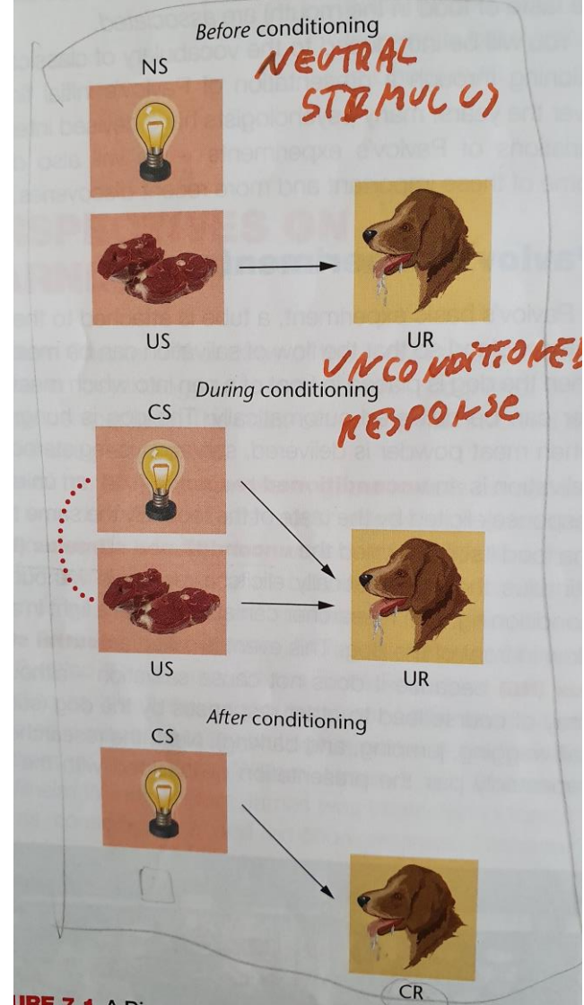
FIGURE 7.1 A Diagram of Classical Conditioning. Before conditioning, the unconditioned stimulus (US) causes the unconditioned response (UR) – this does not have to be learned. A neutral stimulus (NS) does not cause a response.
